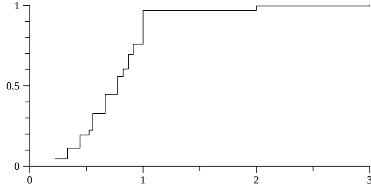
Fig. 2 CDF of the measurement errors defined in (17).
