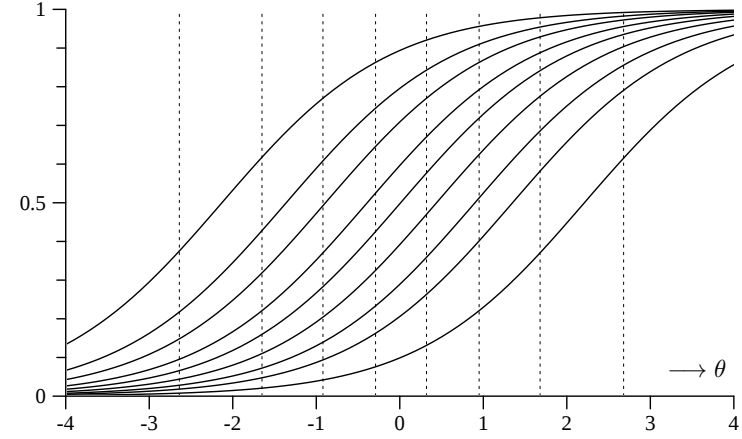
Fig. 7 The functions L(\theta - \delta_j^*) and values of \theta^*(s^c) , based on Table (39).
