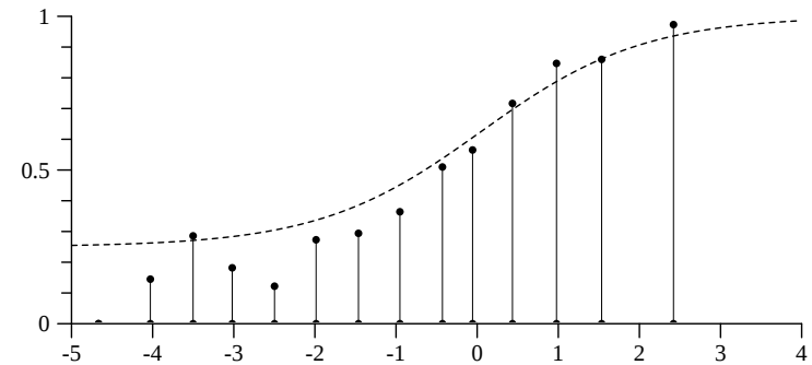
Fig. 15 ICC for MC item j = 2 from the model with \gamma = 0.25 . The vertical lines indicate the proportion of correct answers to this item in 14 intervals on the abscissa.
