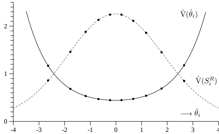
Fig. 11 Based on the 11 non-MC items of the math test, for s_i = 1, \dots, 10 and \hat{\theta}_i = \hat{h}^{-1}(s_i) , the solid line shows the estimated variance \hat{V}(\hat{\theta}_i) and the dashed line shows the estimated variance of the corresponding sum score variable.
