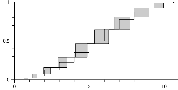
Fig. 4 CDF of the values s_i^c (solid line) and an interval-valued CDF of the estimated expectations based on 11 MC items.
