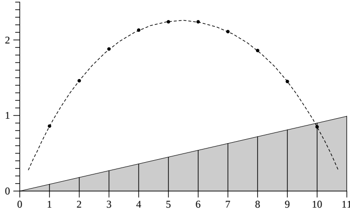
Fig. 10 Based on the 11 non-MC items of the math test, the dashed line shows the function s_i \rightarrow \hat{V}(S_i^R) for s_i = 1, \dots, 10 . The grey-shaded area shows how the intervals V(S_i | S_i^c = s_i^c) , defined in (44), depend on s_i^c = 0, \dots, 11 .
