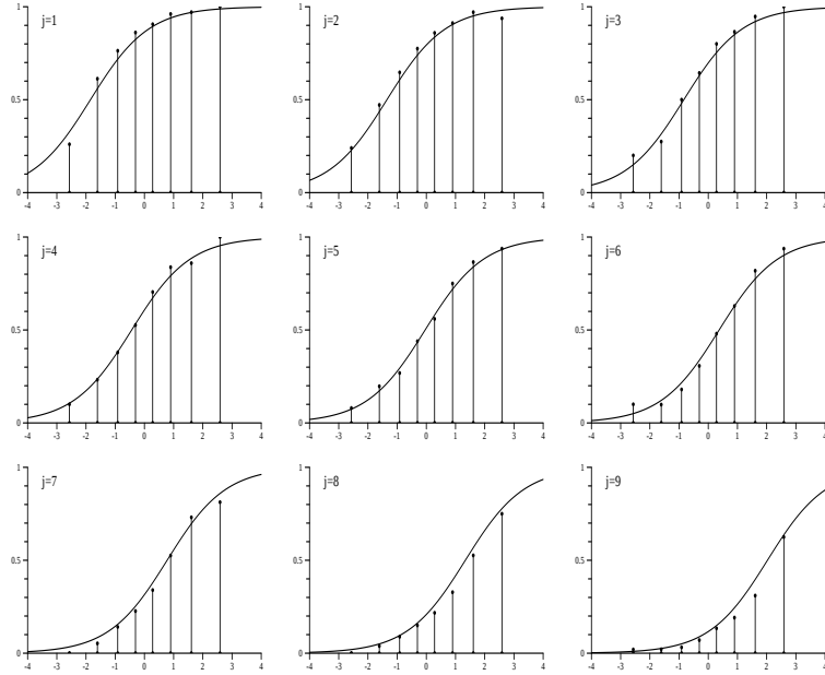
Fig. 9 Estimated ICCs ( \hat{\delta}_j ) and observed proportions P(X_j = 1 | S = s) for s = 1, \dots, 8 and j = 1, \dots, 9 .
