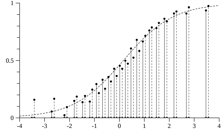
Fig. 12 An ICC centered at 0.16, and proportions of persons who have correctly answered the non-MC item j = 9 (solid) and the MC item j = 11 (dashed).
