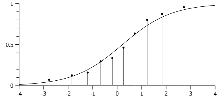
Fig. 14 ICC for MC item j = 2 from the model with \gamma = 0 . The vertical lines indicate the proportion of correct answers to this item for score groups s = 1, \dots, 10 .
