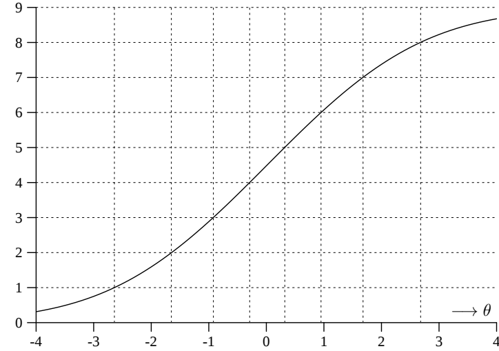
Fig. 8 The function h^*(\theta) and values of \theta^*(s^c) , based on Table (39).
