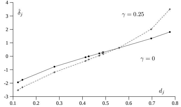
Fig. 13 Comparison of item parameters of 11 MC items of the math test and item difficulties d_j .
