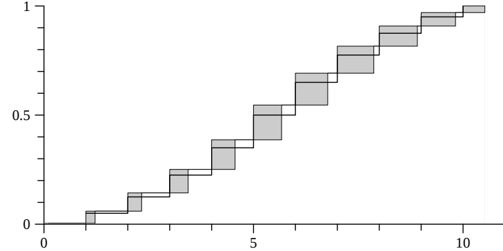
Fig. 1 CDF of the values s_i^c (solid line) and an interval-valued CDF of the estimated expectations based on 11 non-MC items.
