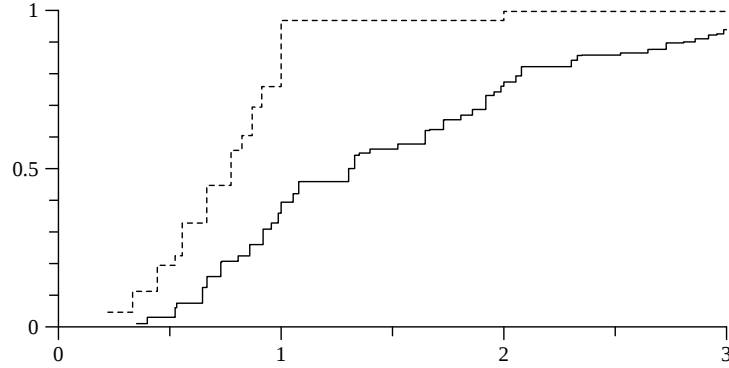
Fig. 5 CDF of the measurement errors defined in (17) for MC items (solid) and non-MC items (dashed, already shown in Figure 2).
