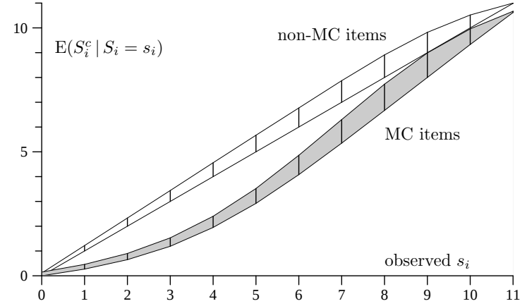
Fig. 3 Illustration of the intervals shown in (16) for non-MC items and in (28) for MC items.
