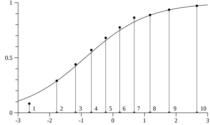
Fig. 6 Comparison of \hat{\pi}_{sj}^R and q_{sj} for j = 7 and s = 1, \dots, 10 .
